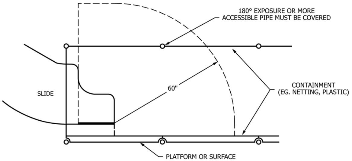
FIG. A1.18 Elevation View Reference Section 8.1.7.2 (2)
