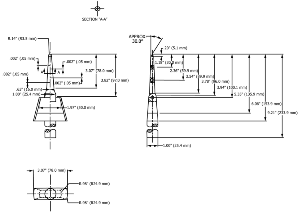
FIG. A1.13 Finger Probe Reference Section 6.6.1.1
