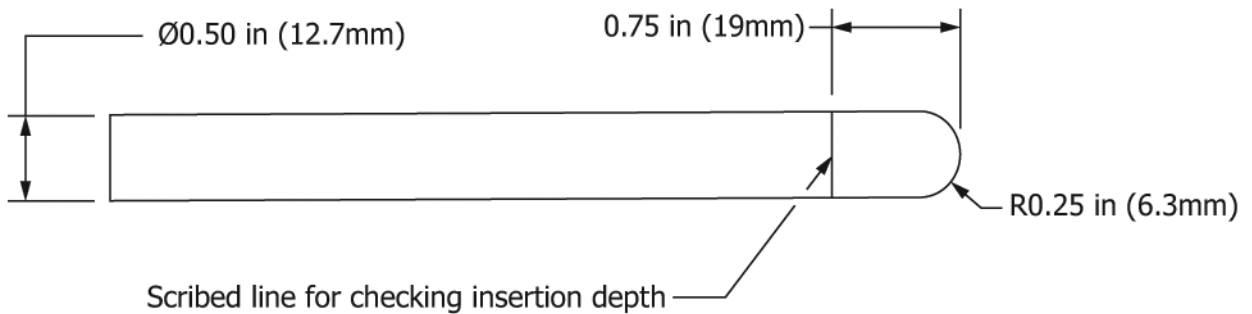
FIG. A1.15 0.50-in. Diameter Test Probe Reference Section 8.1.6.1 (2)
